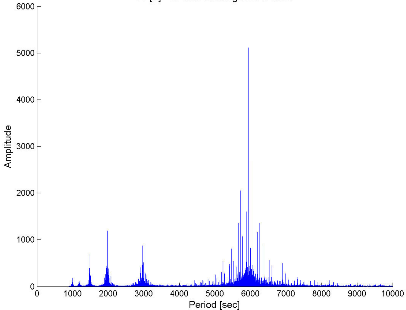
FP[V] - TPMU Periodogram All Data
