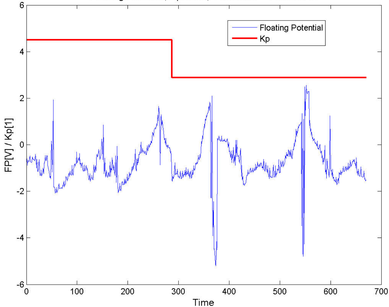
Floating Potential, Kp index, 14/07/2012 - 17/07/2012
