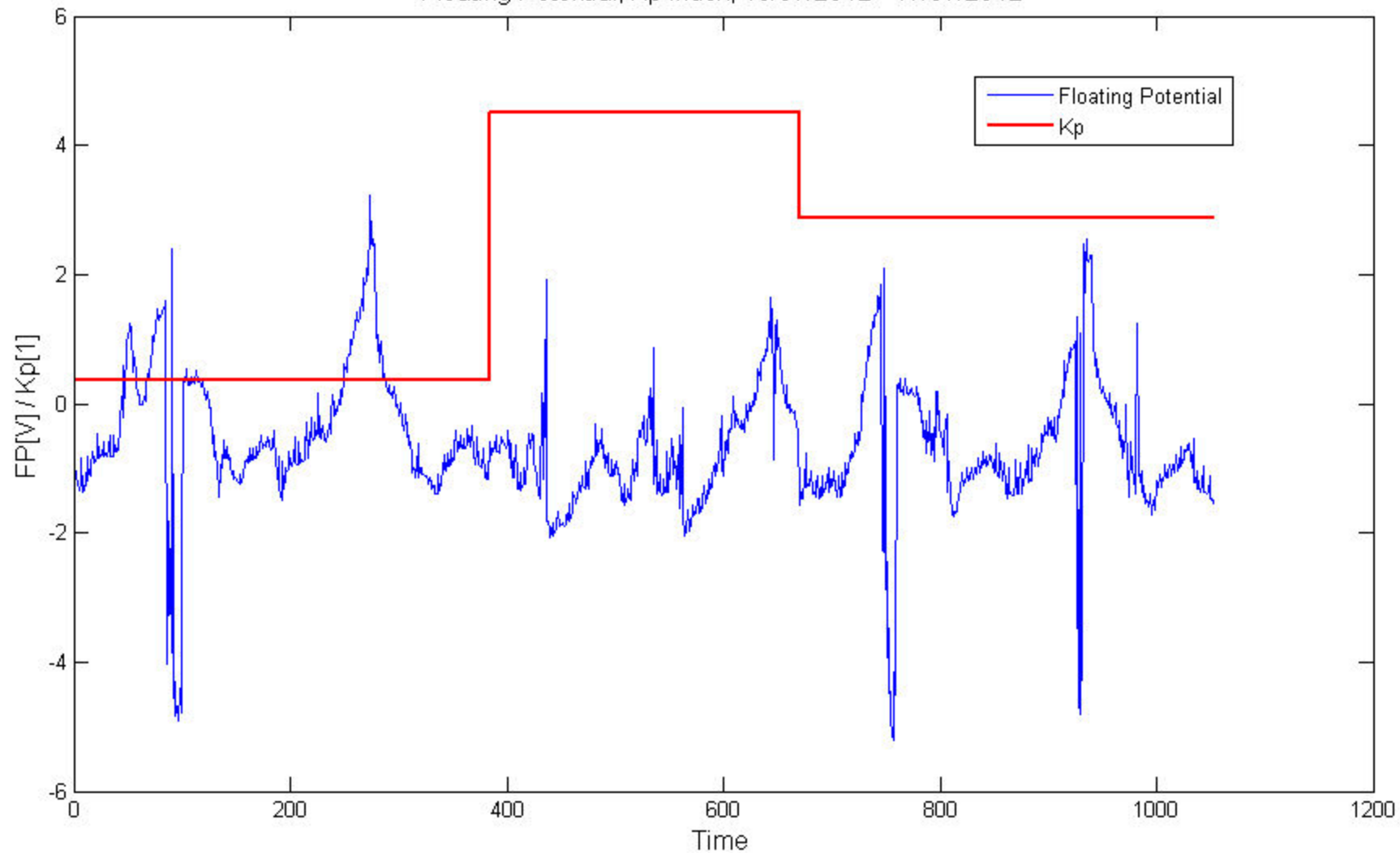
Floating Potential, Kp index, 13/07/2012 - 17/07/2012
