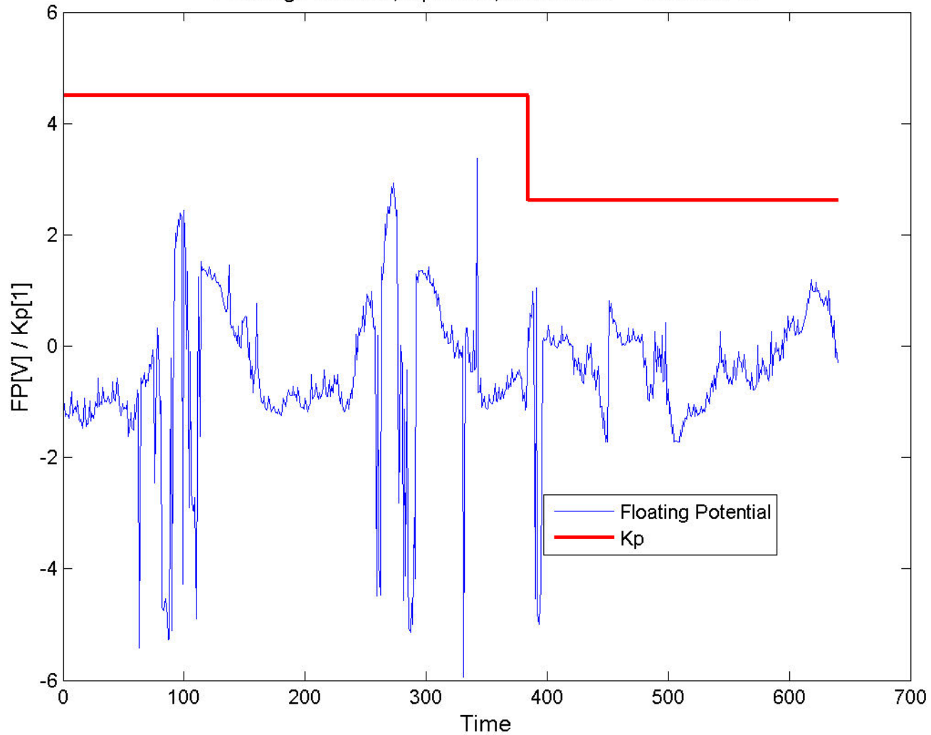
Floating Potential, Kp index, 08/07/2012 - 10/07/2012
